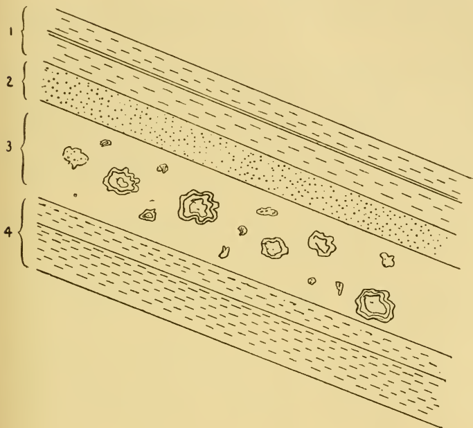
Fig. 1.—SECTION OF LIMESTONE CONTAINING SINGATOKE RIVER CAVERN.
