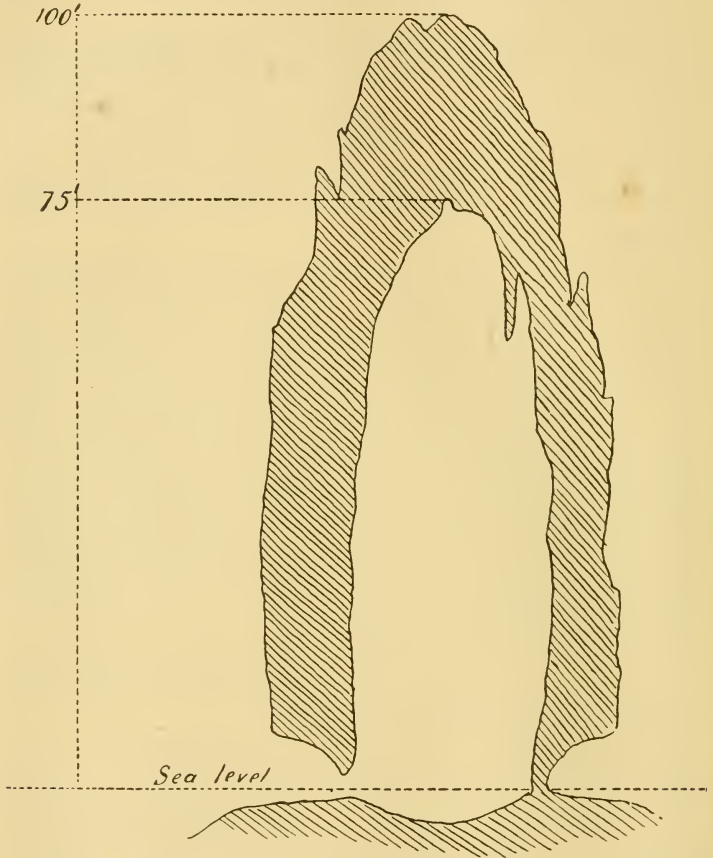
Fig. 2.—SKETCH SECTION OF NGHILLANGHILLAH CAVE.
